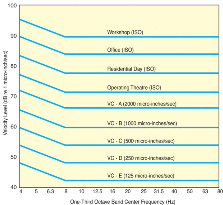
Figure 2 VC curves
