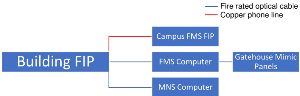
FIGURE 2: CAMPUS WIDE CONNECTIONS BETWEEN BUILDINGS AND FMS
