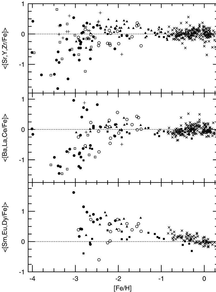
Figure 11 Mean relative abundance ratios of light s -process elements (top panel), heavy s -process elements (middle panel), and r -process elements (bottom panel) as functions of [Fe/H] . In each panel, the dotted horizontal lines represent the solar abundance ratios of these elements. The references for the data points are given in Wallerstein et al. (1997). (We acknowledge C. Sneden for this figure.)
